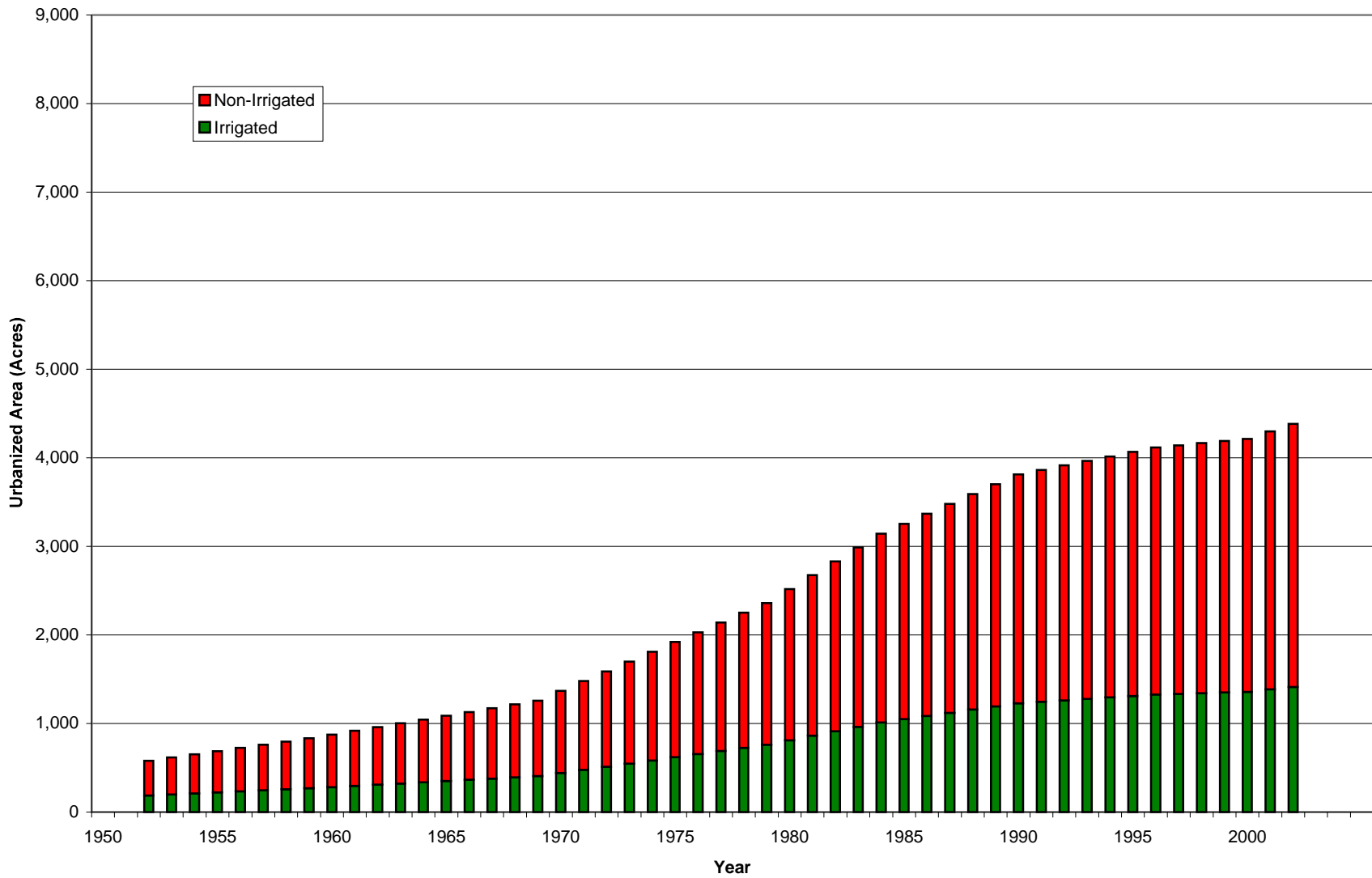
Figure 2.2b Urbanized and Landscaped Area within the Turlock Groundwater Basin, 1952-2002, for Ceres
