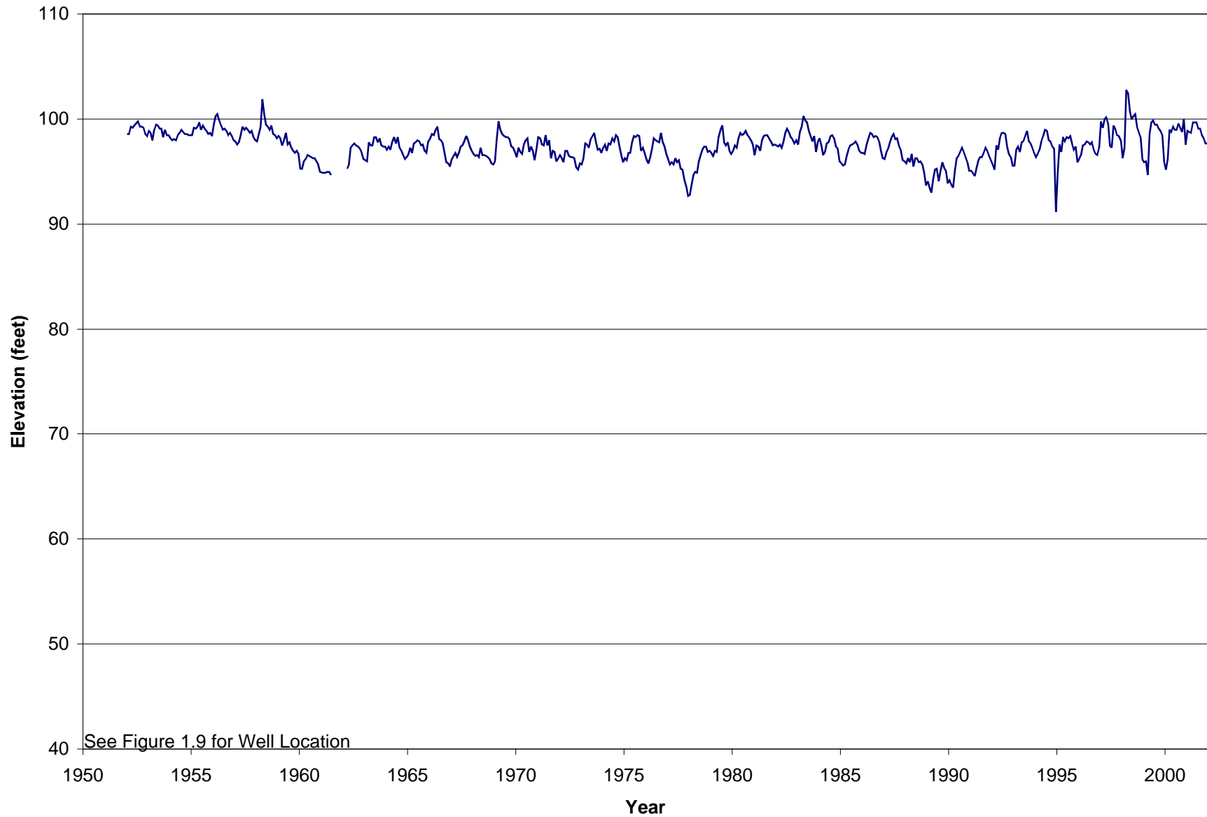
Figure 1.11d Measured Temporal Groundwater Levels in Section-Corner Well 401
