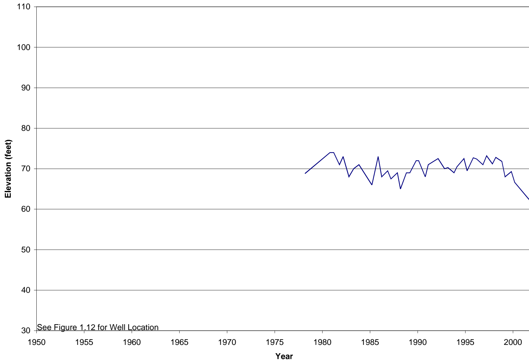
Figure 1.14d Measured Temporal Groundwater Levels in Monitoring Well 06S10E16M001M
