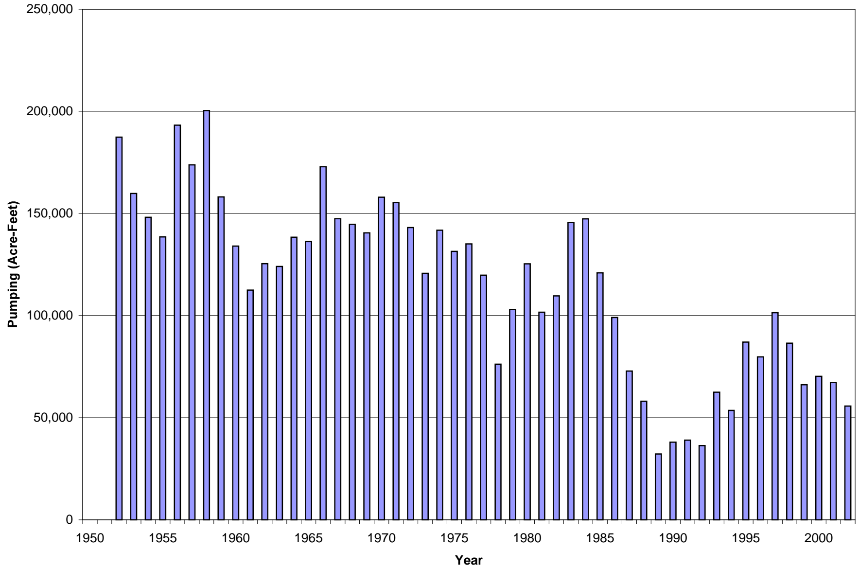
Figure 3.1 Annual Pumpage from Turlock Irrigation District Drainage Wells, 1952-2002
