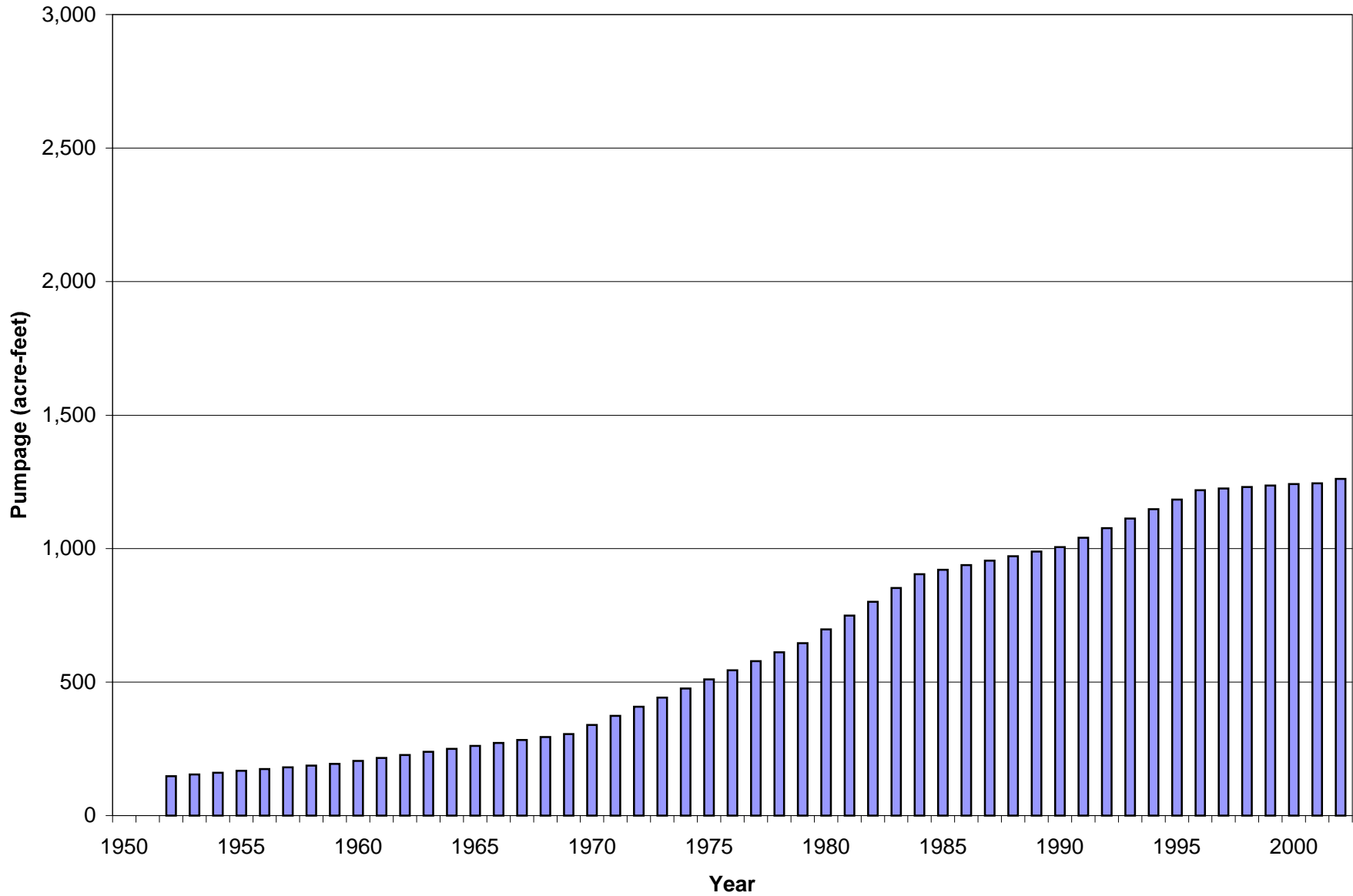
Figure 3.9e Annual Pumpage from Municipal Wells for Hilmar, 1952-2002
