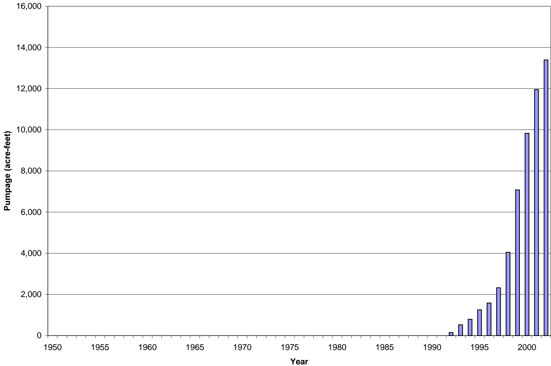
Figure 3.4 Annual Pumpage from Primary-Source Private Irrigation Wells within Turlock Irrigation District, 1952-2002
