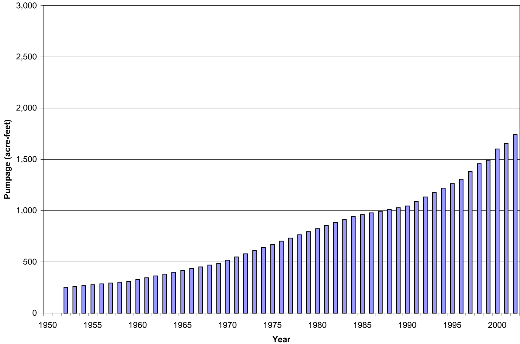
Figure 3.9b Annual Pumpage from Municipal Wells for Delhi, 1952-2002
