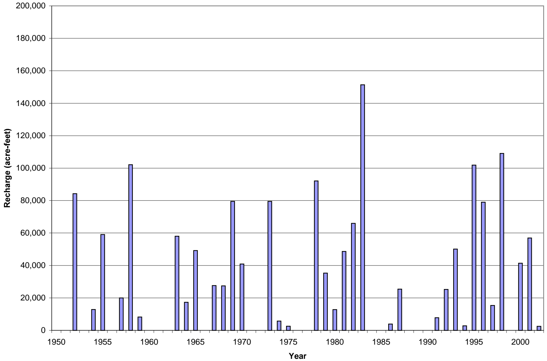
Figure 4.9 Annual Recharge from Non-Irrigated Areas, 1952-2002
