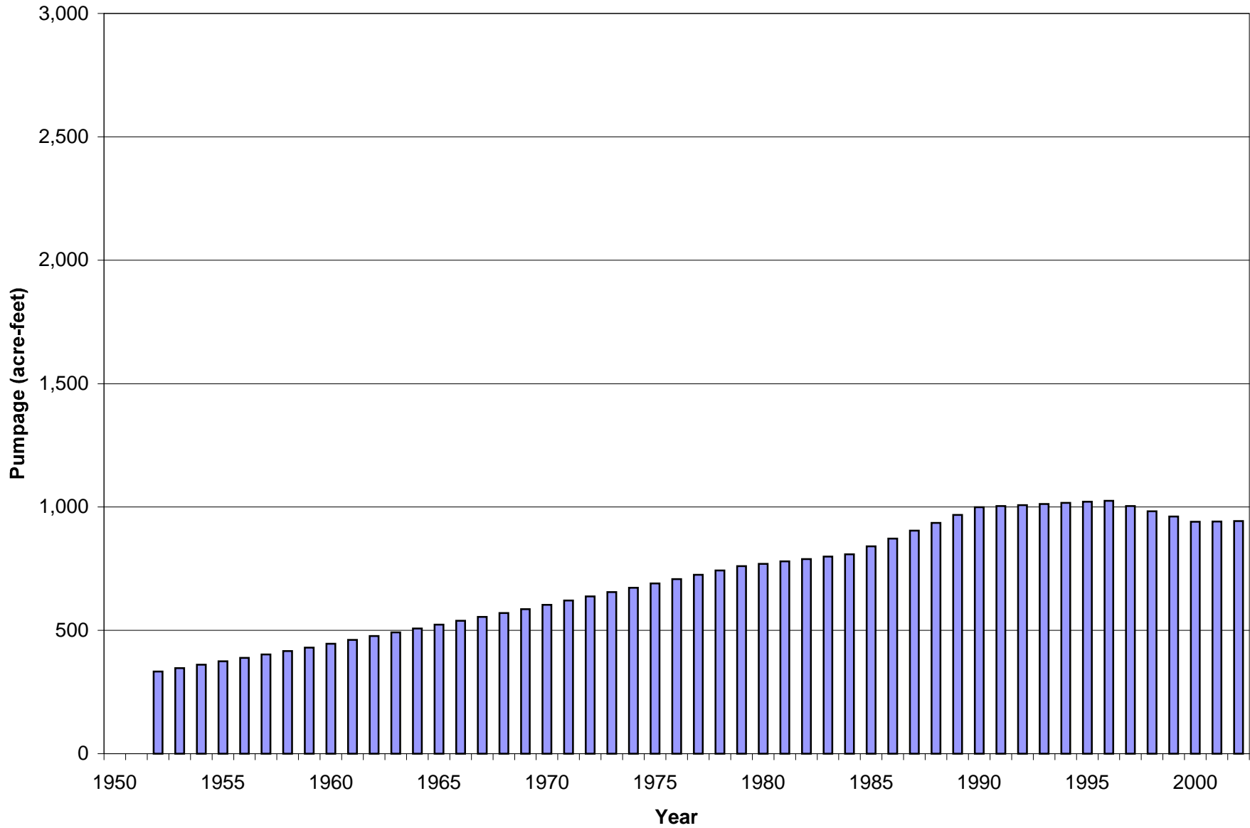
Figure 3.9f Annual Pumpage from Municipal Wells for Hughson, 1952-2002
