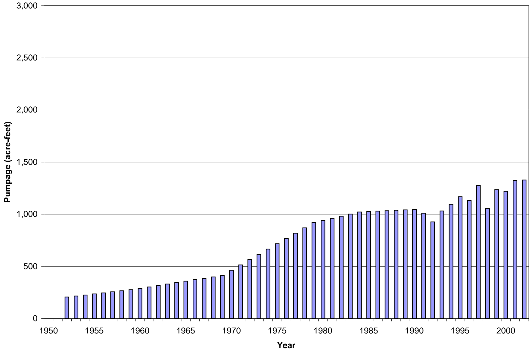
Figure 3.9c Annual Pumpage from Municipal Wells for Denair, 1952-2002
