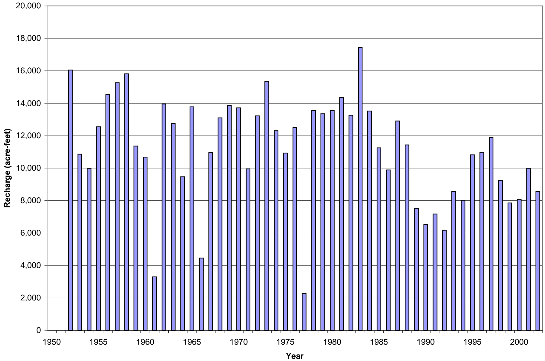
Figure 4.5 Annual Recharge from Merced Irrigation District, 1952-2002
