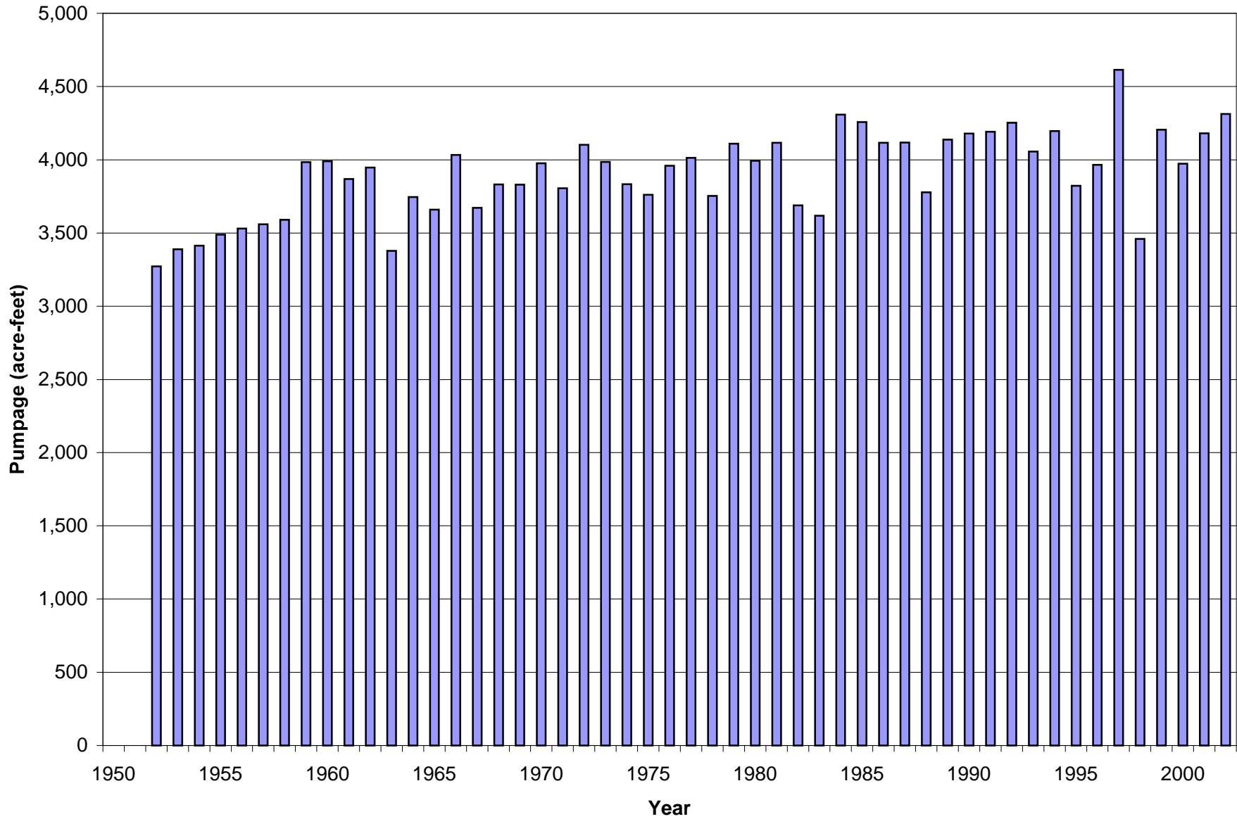
Figure 3.10 Annual Pumpage from Private Domestic Wells, 1952-2002
