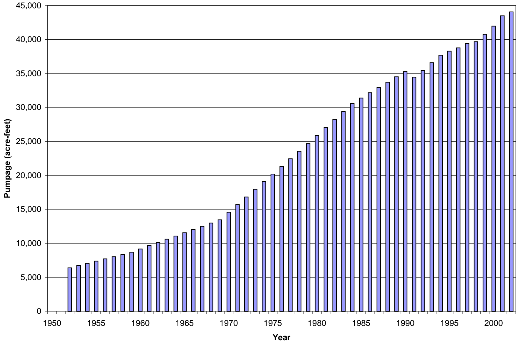
Figure 1.3 Municipal Groundwater Pumping within the Turlock Groundwater Basin, 1952-2002
