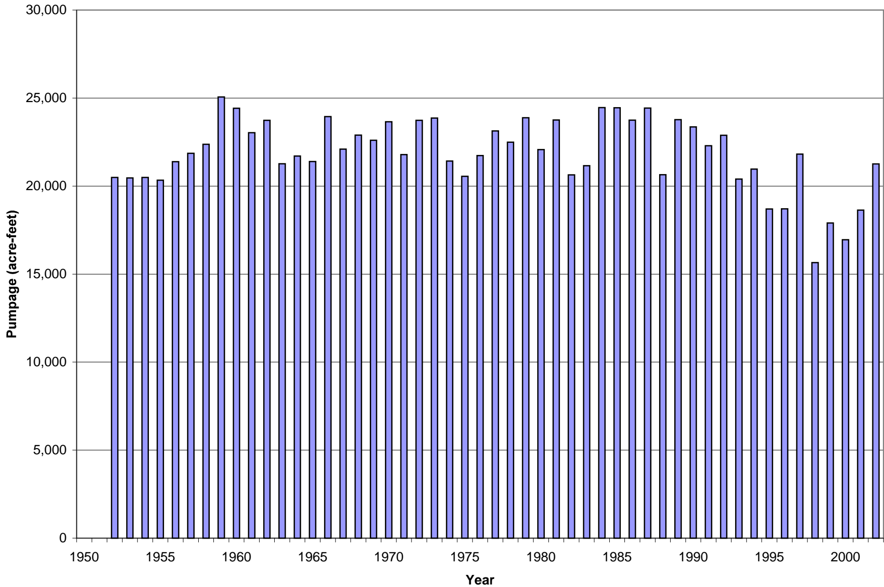
Figure 3.6 Annual Pumpage from Private Irrigation Wells within Ballico-Cortez Water District, 1952-2002
