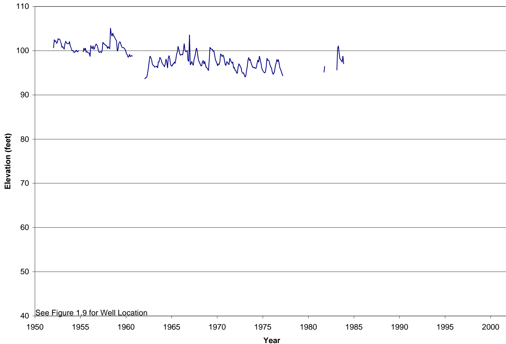
Figure 1.11c Measured Temporal Groundwater Levels in Section-Corner Well 351
