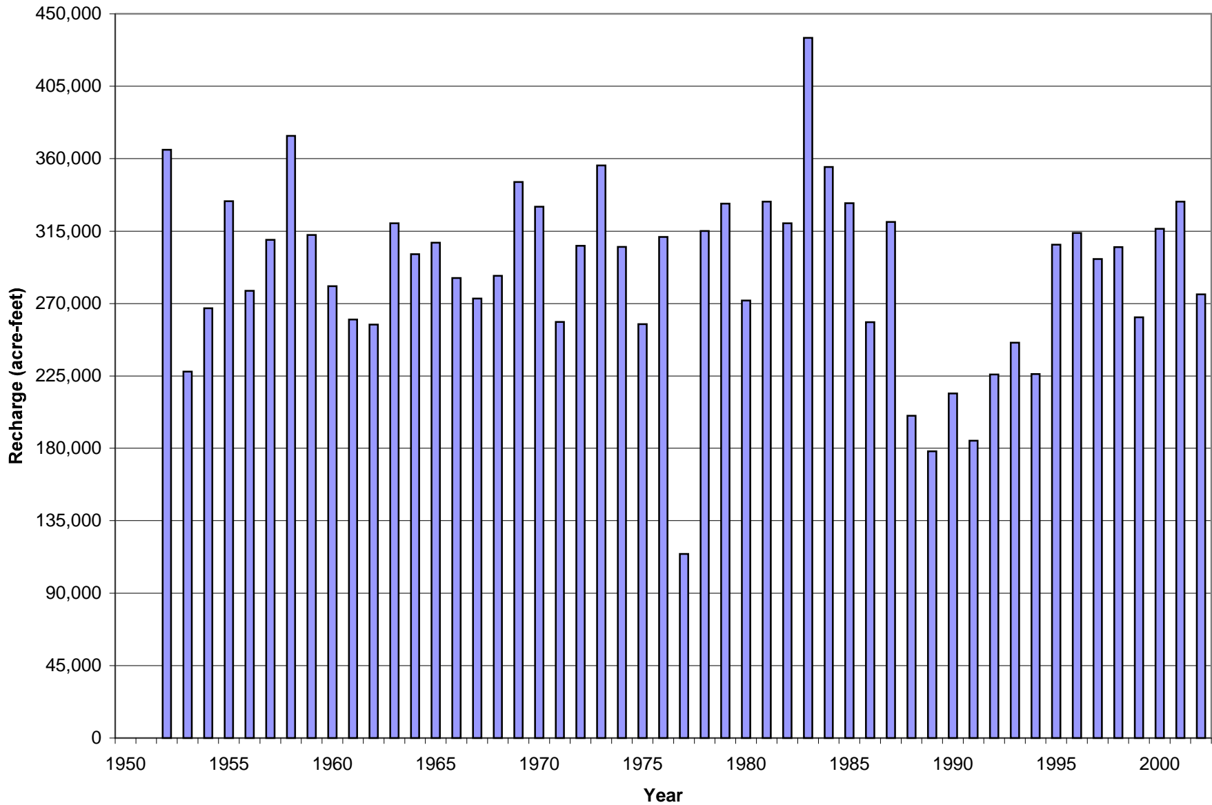
Figure 4.1 Annual Recharge from Turlock Irrigation District Canal-Delivery Lands, 1952-2002
