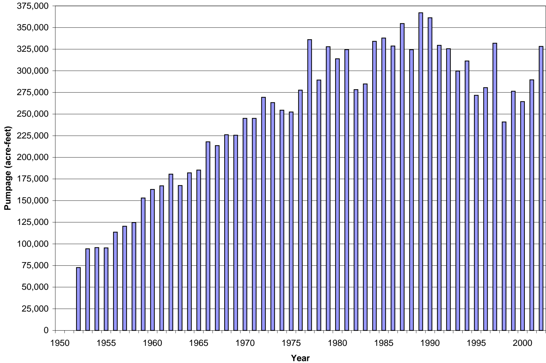
Figure 1.5 Agricultural Groundwater Pumping from Water Districts within the Turlock Groundwater Basin, 1952-2002
