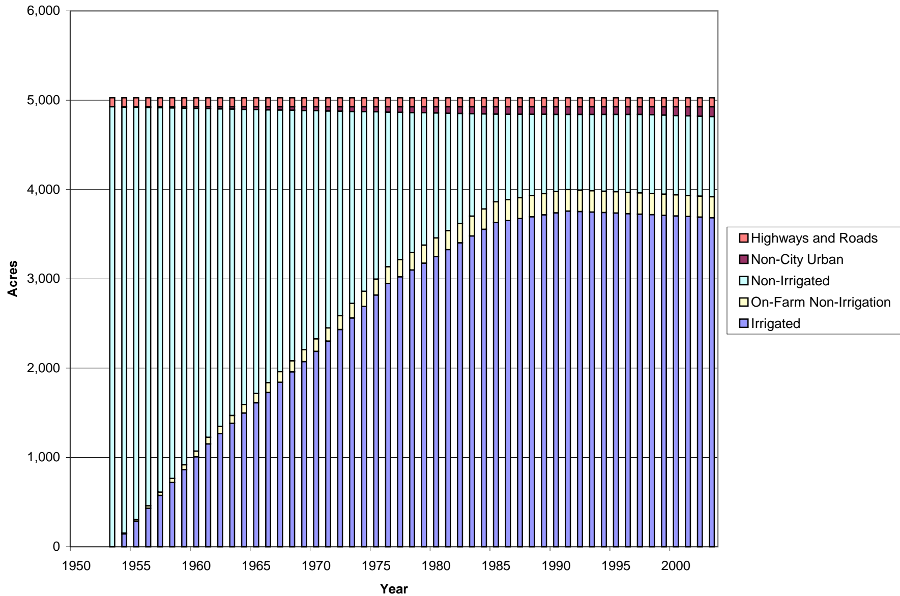
Figure 2.4e Land Use within the Turlock Groundwater Basin, 1952-2002, for Merced River Non-District Area
