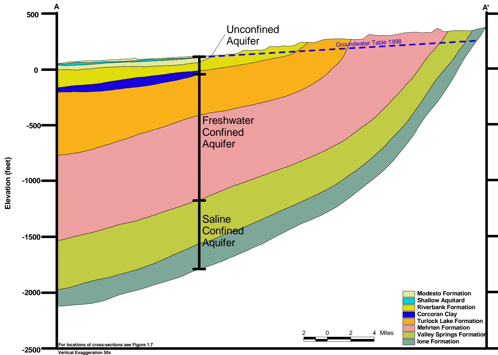
Figure 1.8 East-West Cross-Section Showing Hydrogeologic Units within the Groundwater Basin
