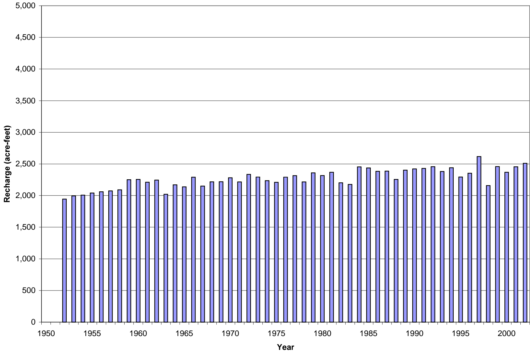
Figure 4.8 Annual Recharge from Rural Residences, 1952-2002
