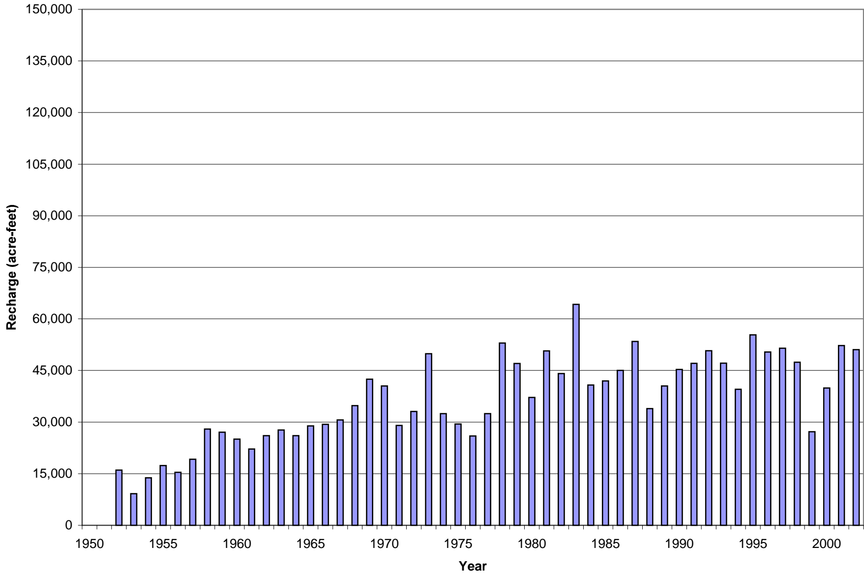
Figure 4.6 Annual Recharge from Non-District Areas, 1952-2002
