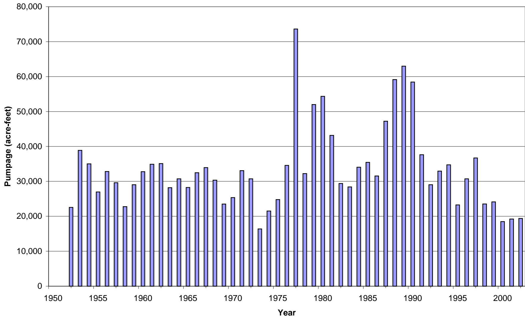
Figure 3.2 Annual Pumpage from Supplemental-Source Private and Improvement District Irrigation Wells Within Turlock Irrigation District, 1952-2002
