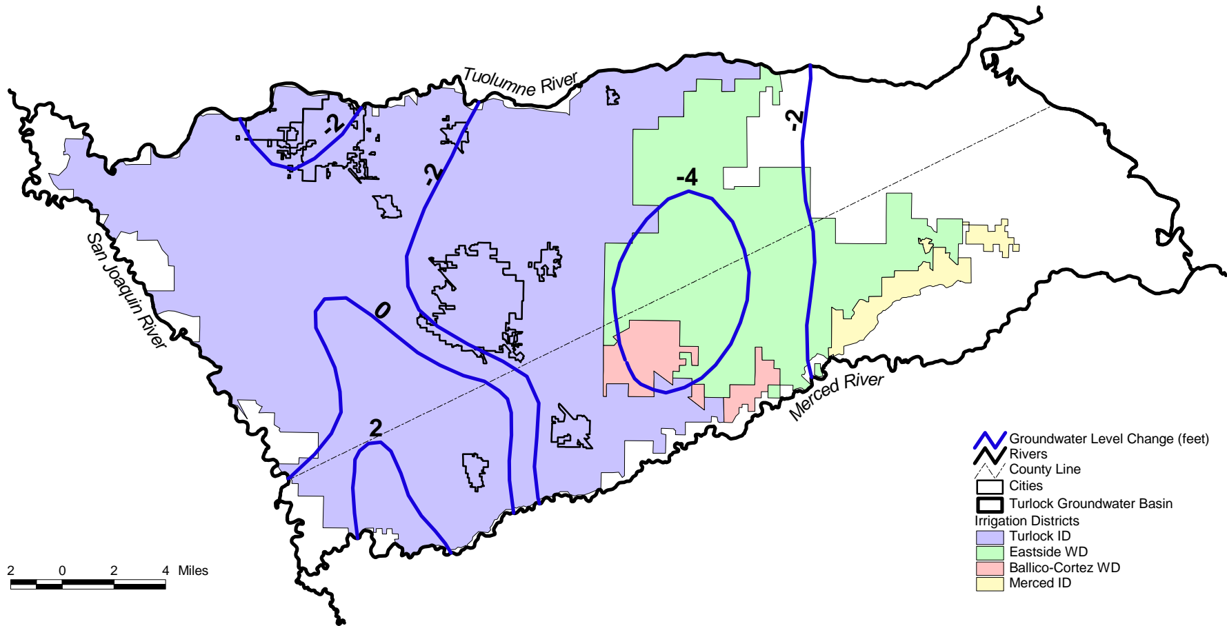
Figure 5.1g Annual Groundwater Level Changes within Turlock Groundwater Basin, 1983-1987
