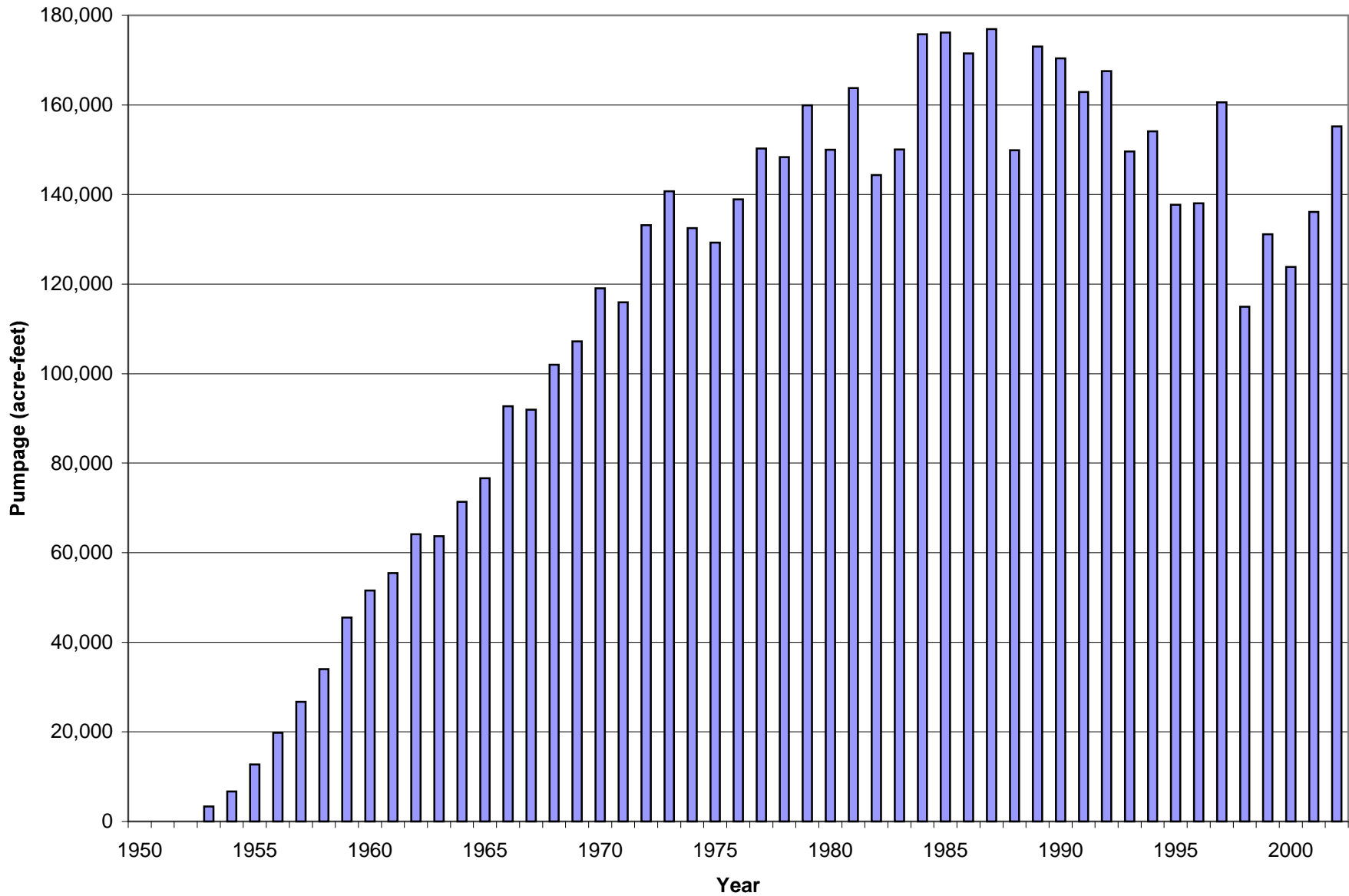
Figure 3.5 Annual Pumpage from Private Irrigation Wells within Eastside Water District, 1952-2002
