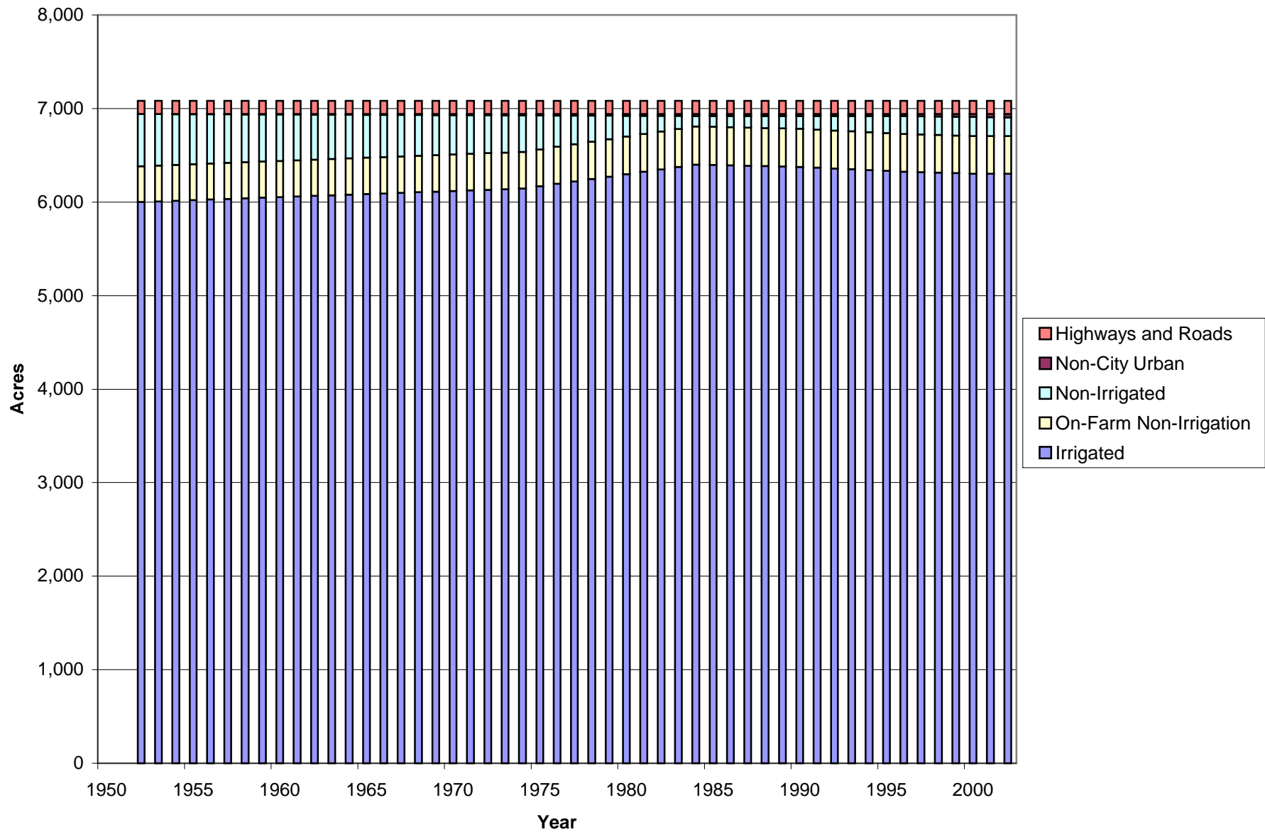
Figure 2.4b Land Use within the Turlock Groundwater Basin, 1952-2002, for Ballico-Cortez Water District
