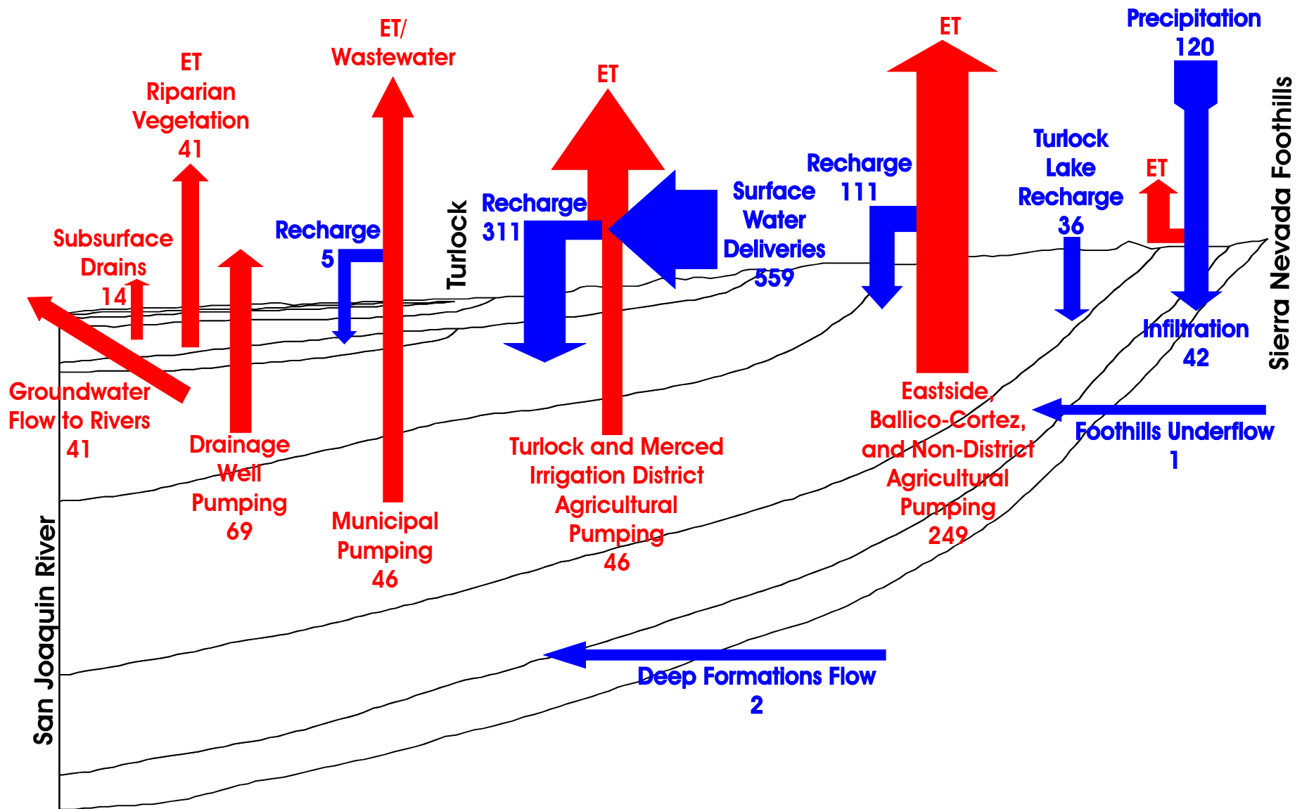
1998-2002 Turlock Groundwater Basin Water Budget (Thousands of Acre-Feet per Year)
